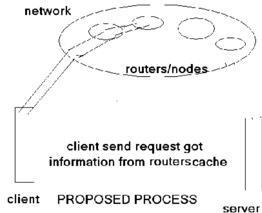
Figure3: Proposed Architecture
