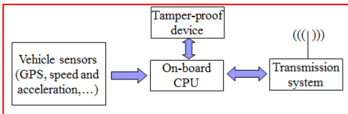
Figure 2:-Tamper proof Device
