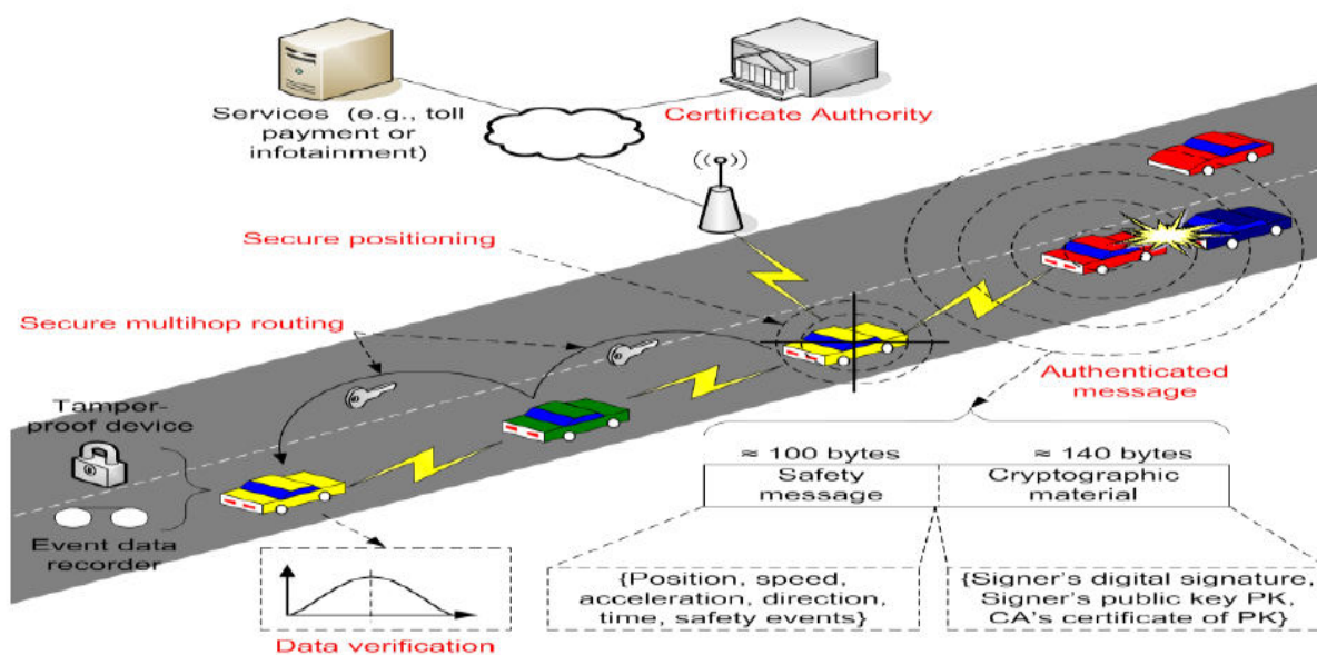
Figure 1:- Security Architecture for VANETs
